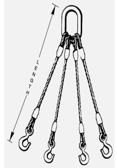
FOUR-LEG SLING
